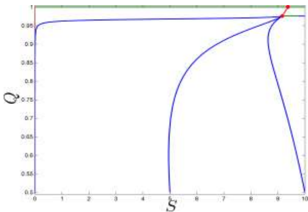
Fig. 4a. The complete state-state diagram in the relevant region in case of low advertising cost ( e=1 )
