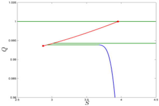
Fig. 5b. The state-state diagram close to the equilibria (red line is a continuum of equilibria)
