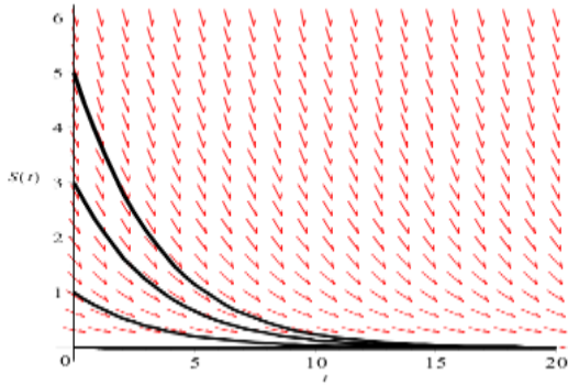
Fig. 3a. Commercial failure ( \delta \geq \kappa )
