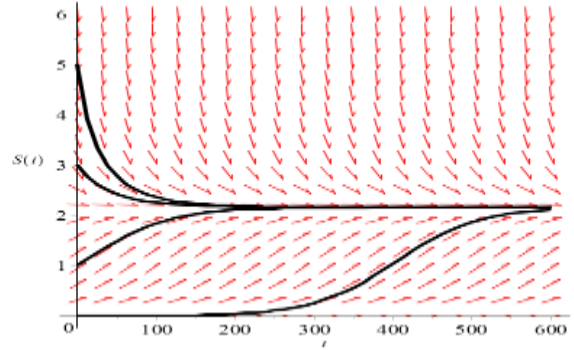
Fig. 3b. Commercial success ( 1 \geq Q_0 > \frac{1 + \beta}{1 + \beta + \kappa - \delta} )
