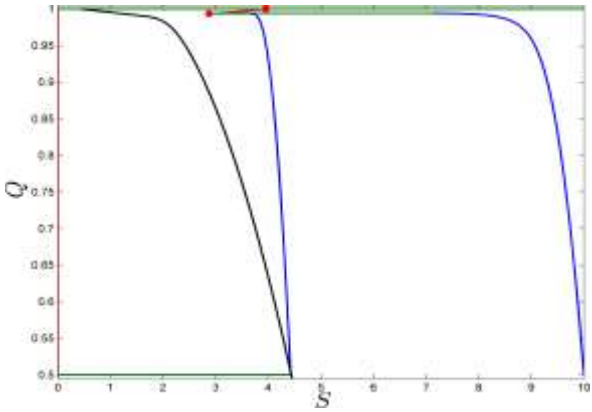
Fig. 5a. The complete state-state diagram in the relevant region in case of intermediate advertising cost ( e=800 )
