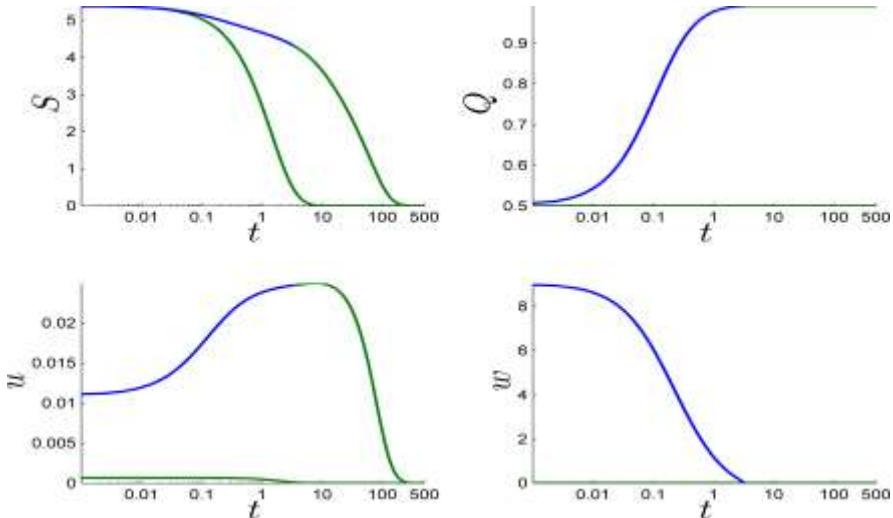
Fig. 6b. The time paths in case of high advertising cost, e=1400 , when S and Q start to the right of the Skiba curve; S approaches zero while Q approaches a high level
