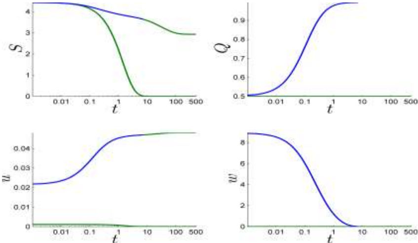
Fig. 5c. The time paths in case of intermediate advertising cost ( e=800 ) when S and Q start close to the Skiba curve
