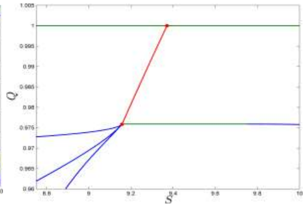
Fig. 4b. The state-state diagram close to the equilibria (red line is a continuum of equilibria)
