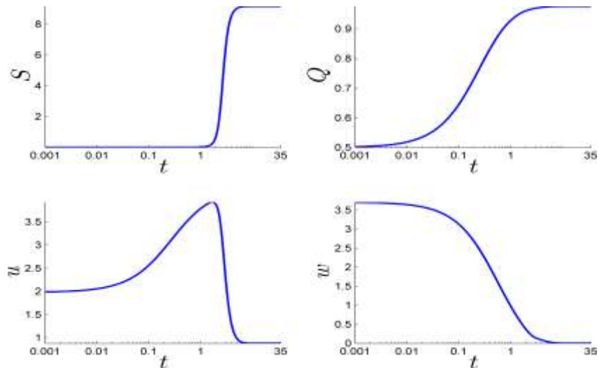
Fig. 4c. The time paths in case of low advertising cost ( e=1 ) when both S and Q start from a low level
