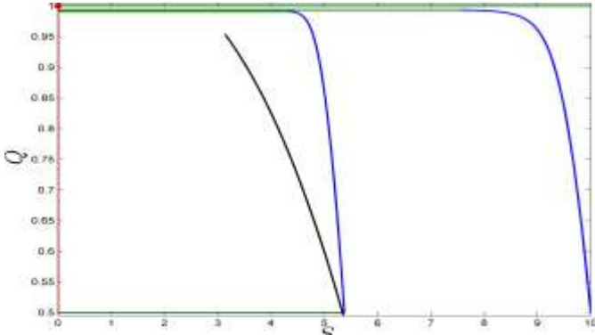
Fig. 6a. The state-state diagram in the relevant region in case of high advertising cost ( e=1400 )
