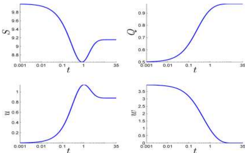
Fig. 4d. The time paths in case of low advertising cost ( e=1 ) when S start from a high level and Q start from a low level
