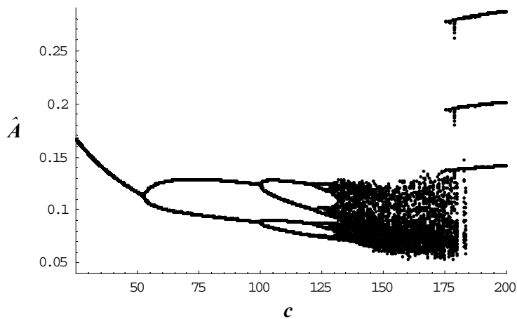
Figure 4: Bifurcation diagram of parameter c for a = 0.2 , b = 0.39 , \alpha = 0.2799 and \beta = 0.458 . Initial conditions are given by A_0 = D_0/2 = 0.13 .
