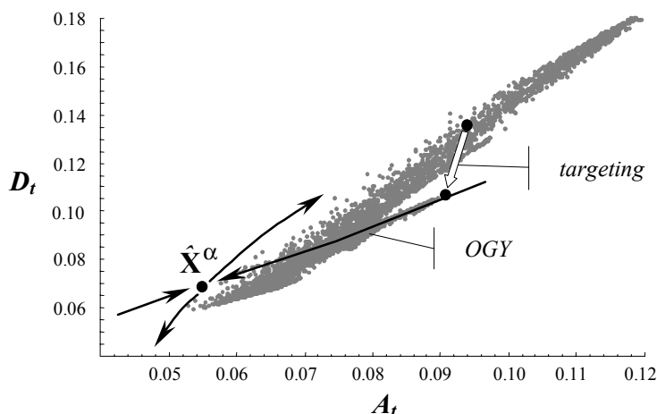
Figure 5: Chaotic attractor, unstable one-period fixed point and its stable and unstable directions, respectively, of System (1) and (2) for a = 0.2 , b = 0.39 , \alpha = 0.2977 , \beta = 0.458 and c = 161.1536 . A_0 = D_0/2 = 0.13 and the time horizon is equal to t = 50, \dots, 5,000 .
